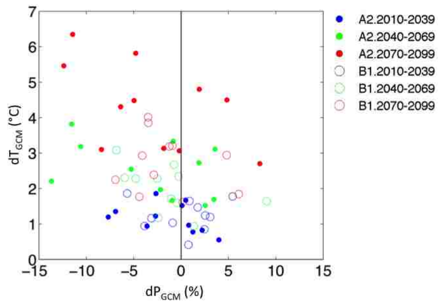
FIG 3.3 Temperature ( dT ) and Precipitation ( dP ) changes for GCMs used in Chistensen and Lettenmaier (2007)
