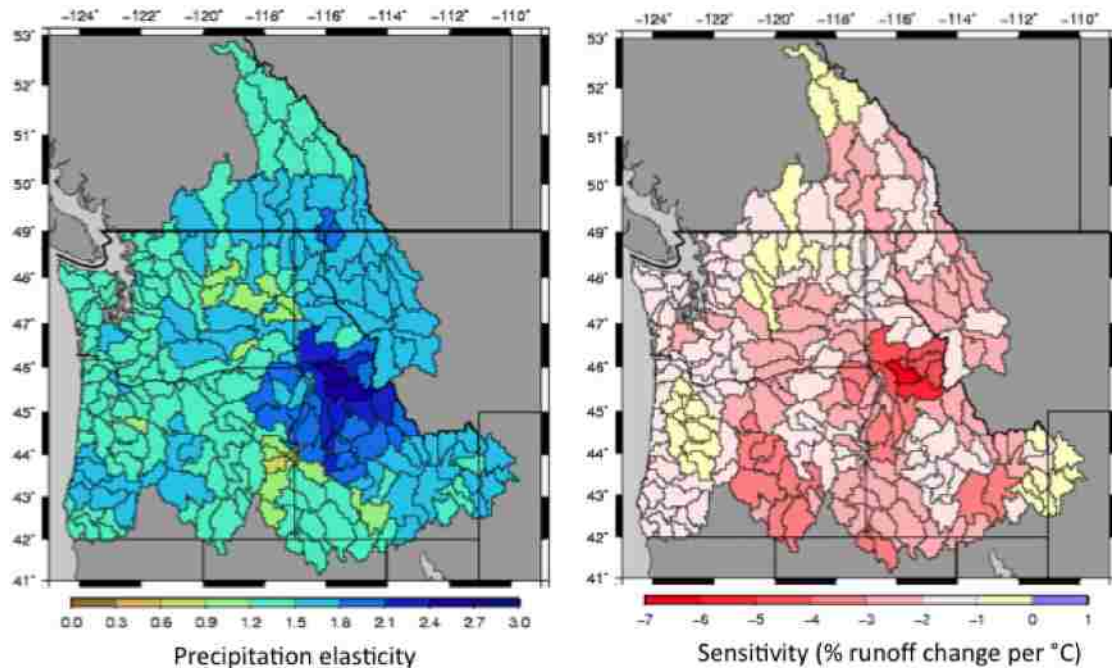
FIG 4.5 Watershed scale annual precipitation elasticities ( \epsilon ) and temperature sensitivities (S). Annual responses (percent) to annually applied change (percent precipitation change or ^{\circ}\text{C} warming)
